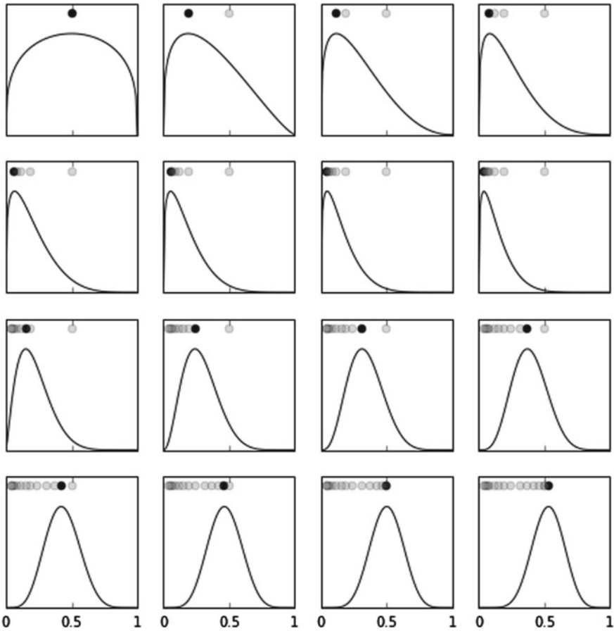
Fig. 3.18 For this example, the prior probability is the \beta(1.3, 1.3) distribution, which has a wider main lobe than the \beta(6, 6) distribution. The dots near the peaks of each of the subgraphs indicate the MAP estimate at that frame
