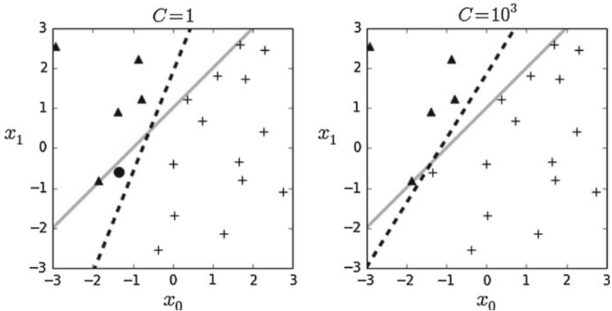
Fig. 4.26 The left panel shows the resulting boundary ( dashed line ) with C = 1 as the regularization parameter. The right panel is for C = 1000 . The gray line is the boundary used to assign the class membership for the synthetic data. The dark circle is the point that logistic regression categorizes incorrectly
