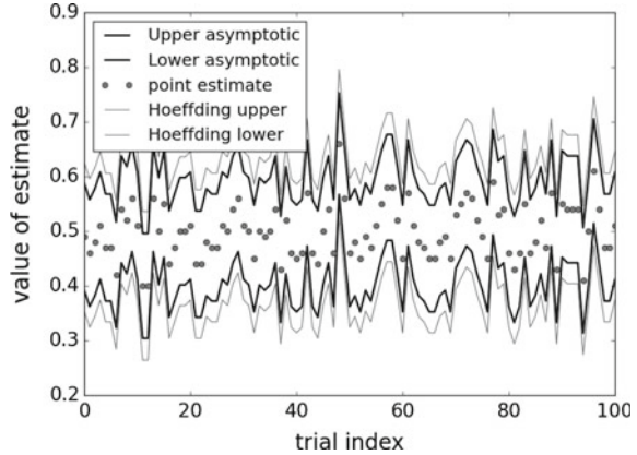
Fig. 3.11 The gray circles are the point estimates and are bounded above and below by both asymptotic confidence intervals and Hoeffding intervals. The asymptotic intervals are tighter because the underpinning asymptotic assumptions are valid for these estimates
