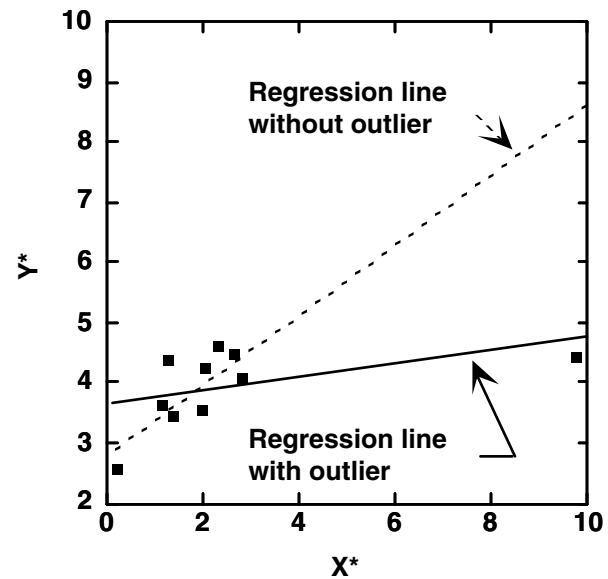
b) outlier with high leverage and high influence
