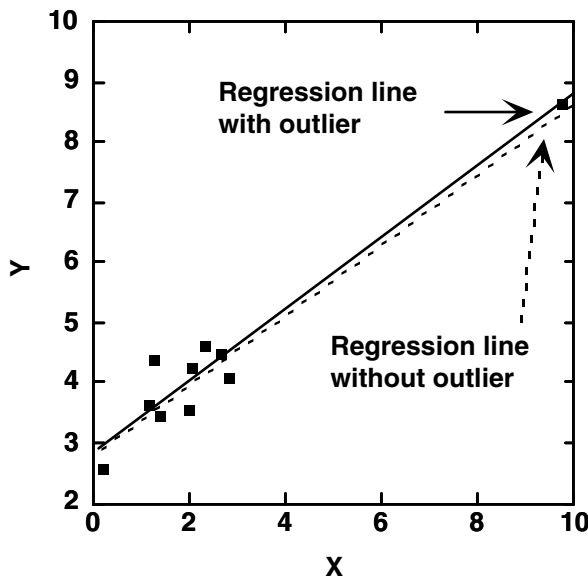
a) outlier with high leverage, but low influence
