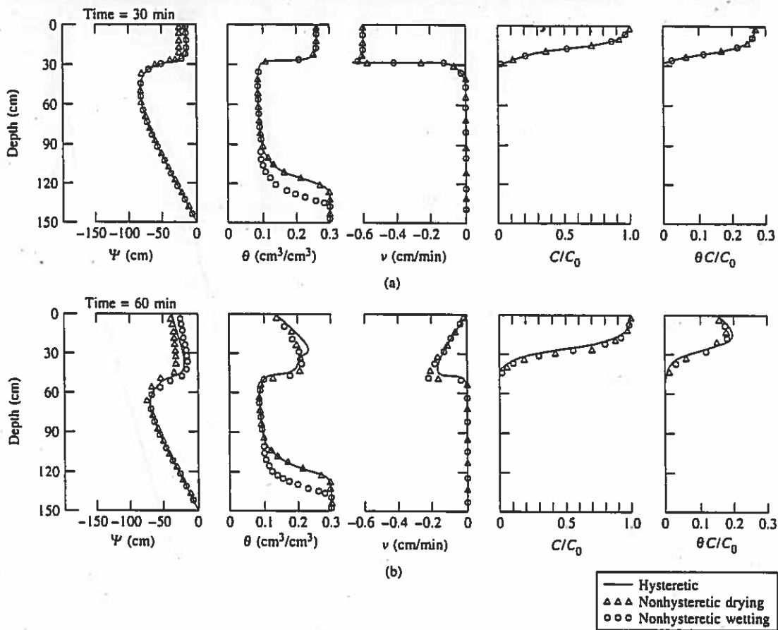
FIGURE 4.17 Model results of matric potential \Psi , water content \theta , pore-water velocity ( v ), relative solute concentration ( C/C_0 ), and volumetric solute concentration ( \theta C/C_0 ). Source: J. F. Pickens and R. W. Gillham, Water Resources Research 16, no. 6 (1980):1071-78. Copyright by the American Geophysical Union.
