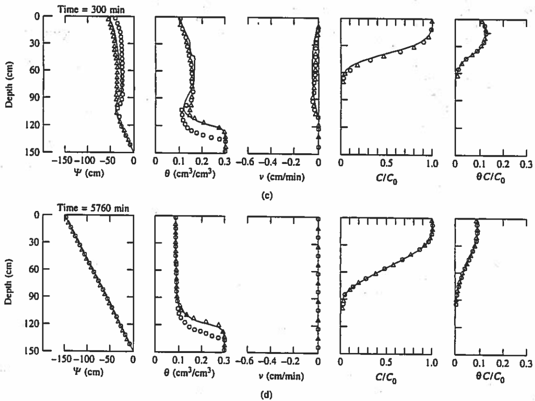
FIGURE 4.17 Model results of matric potential \Psi , water content \theta , pore-water velocity ( v ), relative solute concentration ( C/C_0 ), and volumetric solute concentration ( \theta C/C_0 ). Source: J. F. Pickens and R. W. Gillham, Water Resources Research 16, no. 6 (1980):1071-78. Copyright by the American Geophysical Union.
