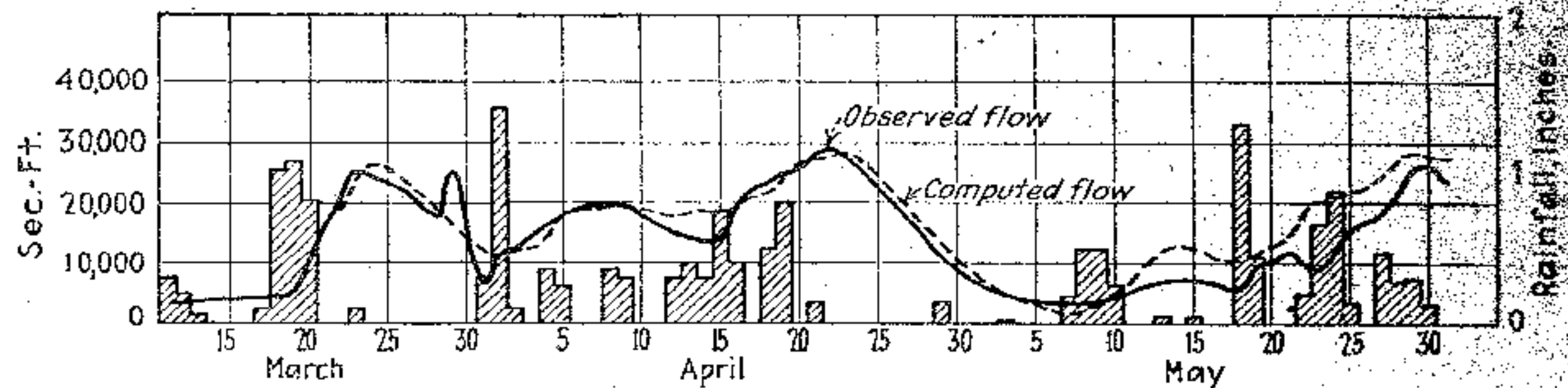
Fig. 5—Close agreement between the computed and observed hydrographs for the Sangamon River at Oakford, Ill., for a three-month period in 1927. Computed flow was based on data recorded in 1922.
