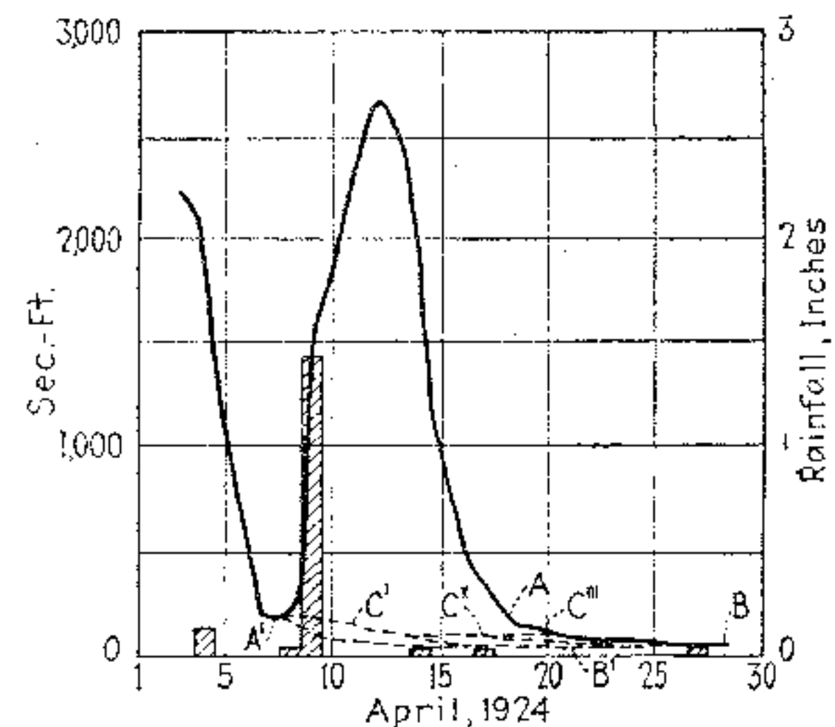
Fig. 2—At Plumfield, Ill., on the Big Muddy River, there was a fairly well-isolated rain of 1.42 in. on April 9, 1924, yielding a hydrograph with ordinates proportional to those of the unit graph.
