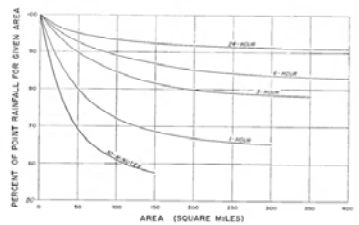
FIGURE 15.—Area-depth curves.
