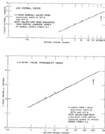
FIGURE 13.—Example of extrapolating to long return periods.
