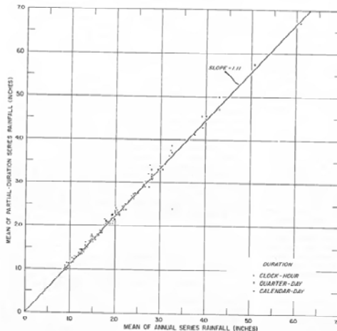
FIGURE 6.—Relation between partial-duration and annual series.
