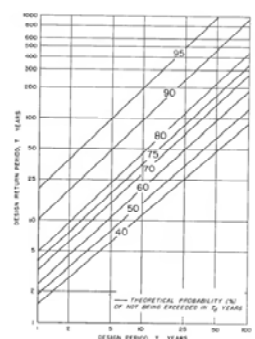
FIGURE 14.—Relationship between design return period, T_d years, design period, T_s years, and probability of not being exceeded in T_s years.
