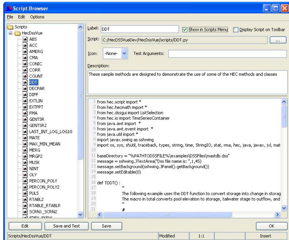
Figure 4.27 Script Editor
