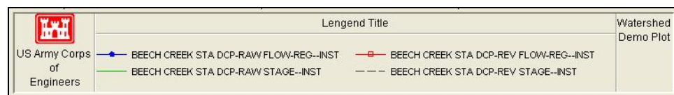
Figure 6.41 Customizing Legends
