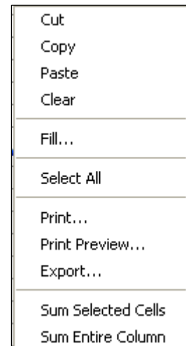
Figure 3.12 Shortcut Menu
