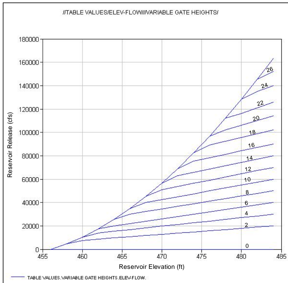
Figure 8.16 Example of two variable rating table paired data, reservoir release as a function of reservoir elevation and gate opening height (curve labels)
