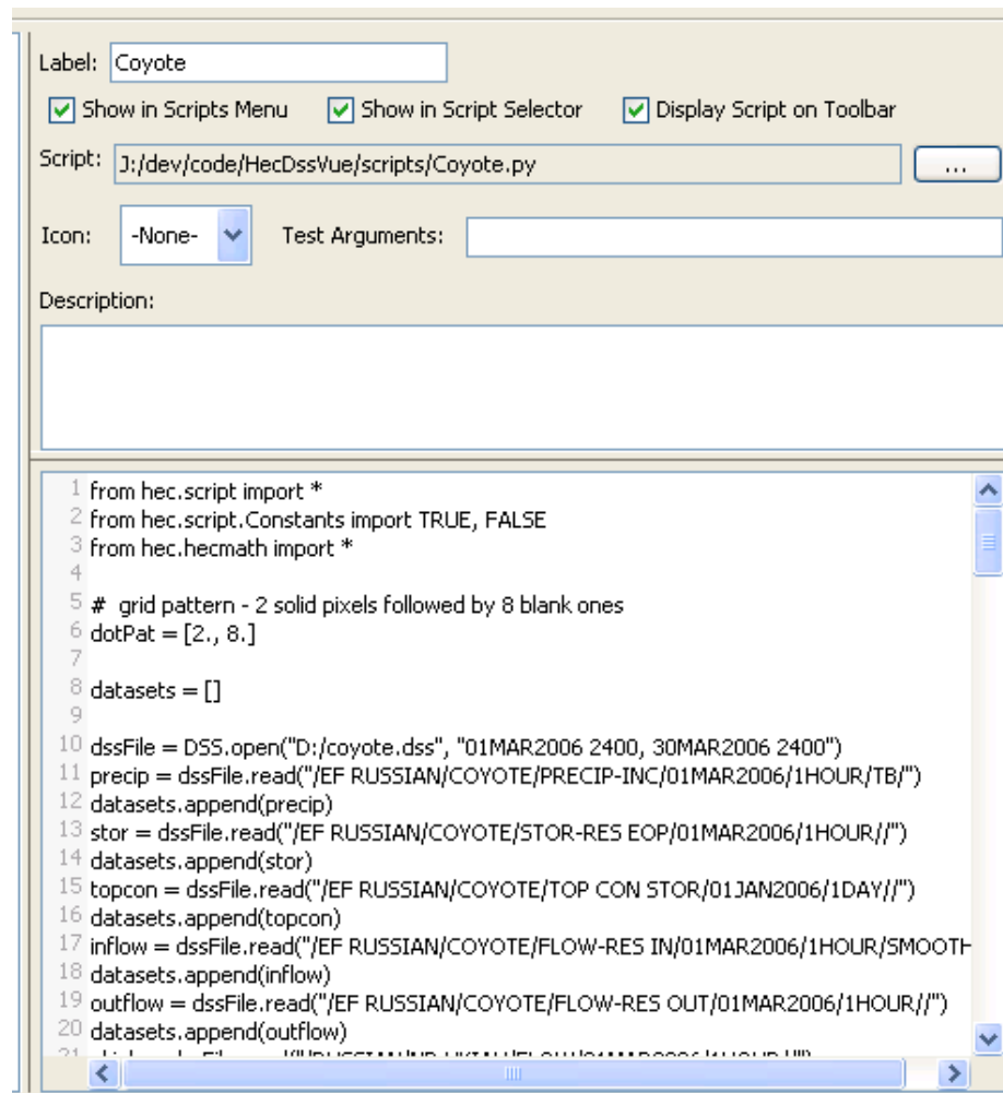
Figure 8.7 Editor Panel
