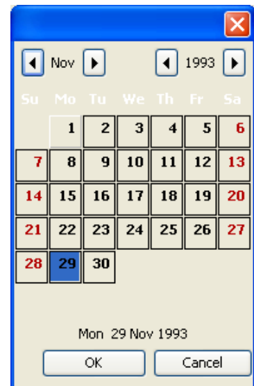
Figure 6.31 Calendar Tool
