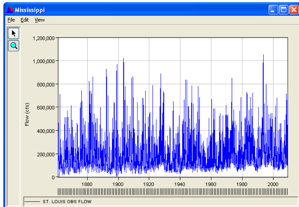
Figure 8.11 Example 17 Results
