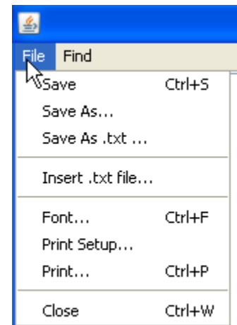
Figure 5.4 File Menu
