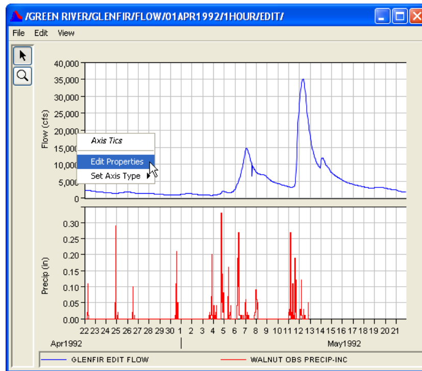
Figure 6.5 Edit Properties
