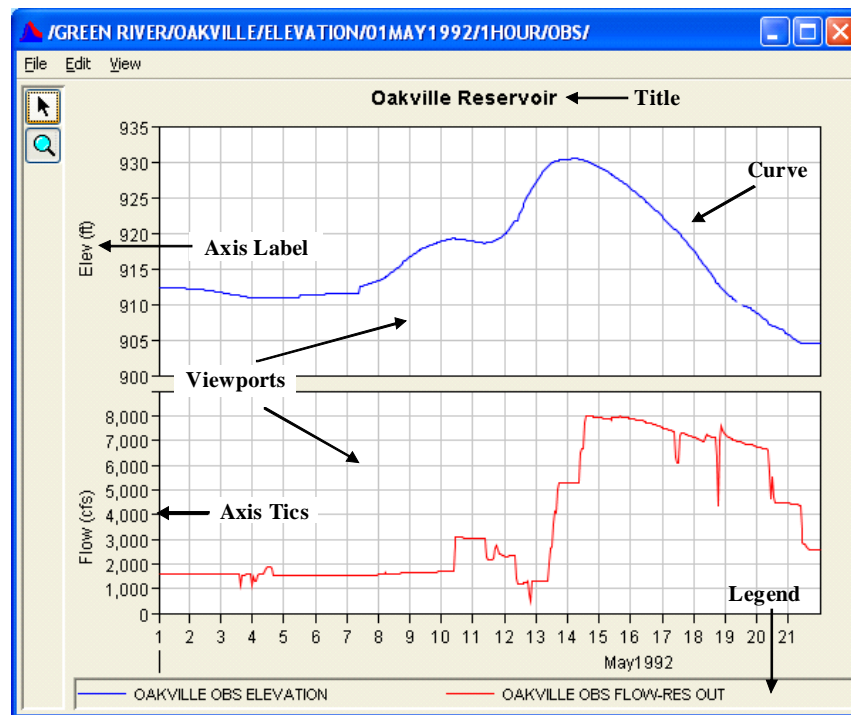
Figure 8.12 Plot Components
