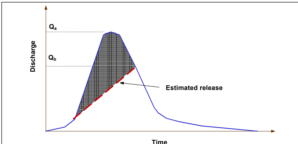
Figure 8.3. Storage volume estimate using actual inflow/estimated release
