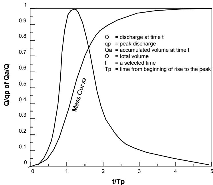
Figure 6.23. Dimensionless unit hydrograph and mass curve
