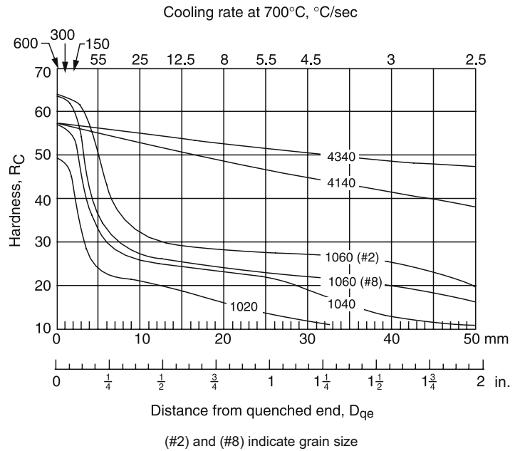
JOMINY HARDENABILITY CURVES FOR SIX STEELS
