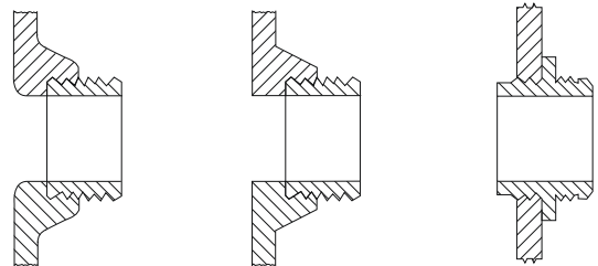
OUTLET SMOOTH AND WELL-ROUNDED COEF. 0.90
