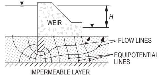
FLOW NET
