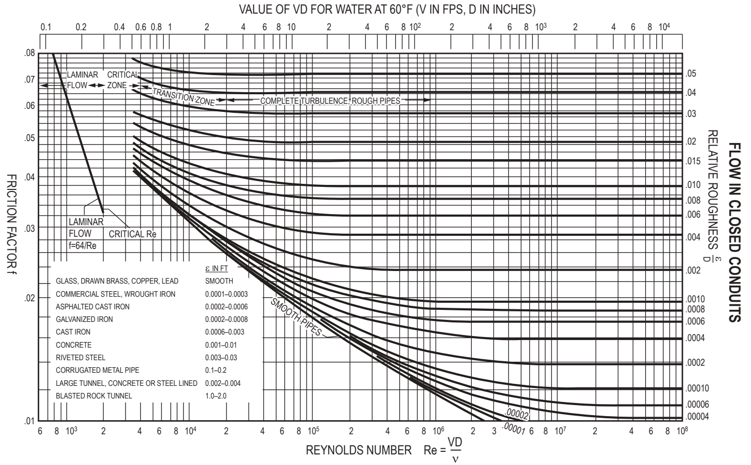
Moody (Stanton) Diagram
