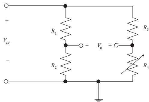
WHEATSTONE BRIDGE
