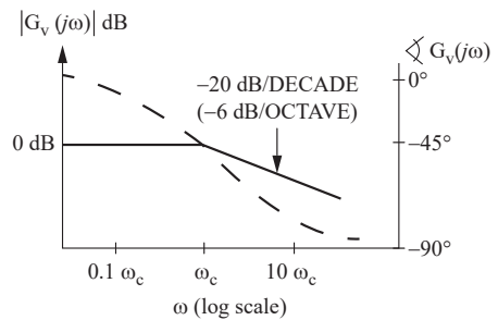
(e) (1 + j\omega/\omega_c)^{-1}
