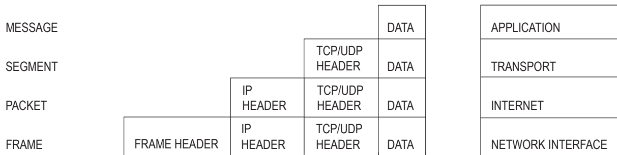
ENCAPSULATION OF APPLICATION DATA THROUGH EACH LAYER
