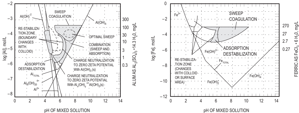
Typical Operating Ranges for Coagulation with Alum and Ferric Chloride
