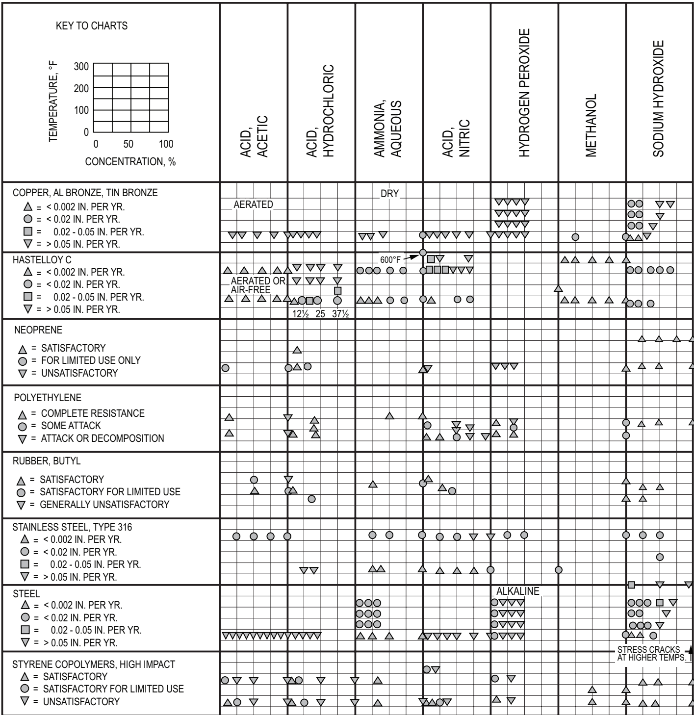
Detailed Corrosion Data on Construction Materials
