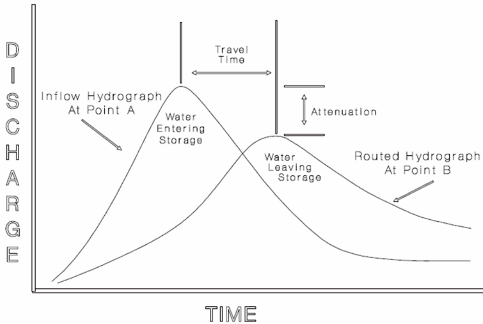
Figure 4-29. Hydrograph routing (USACE 1994)
