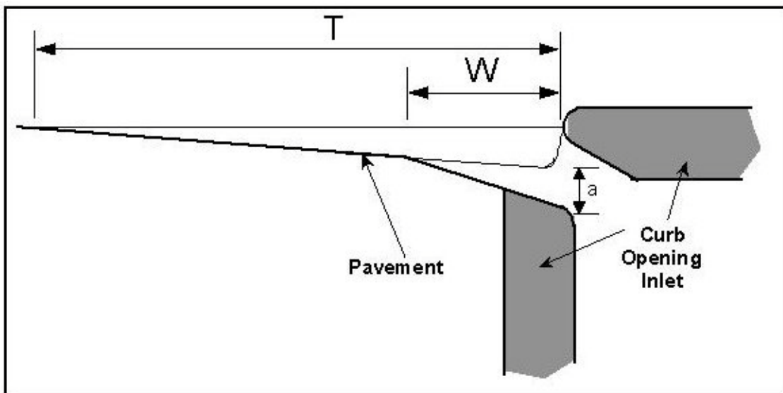
Figure 10-14. Gutter Cross-Section Diagram
