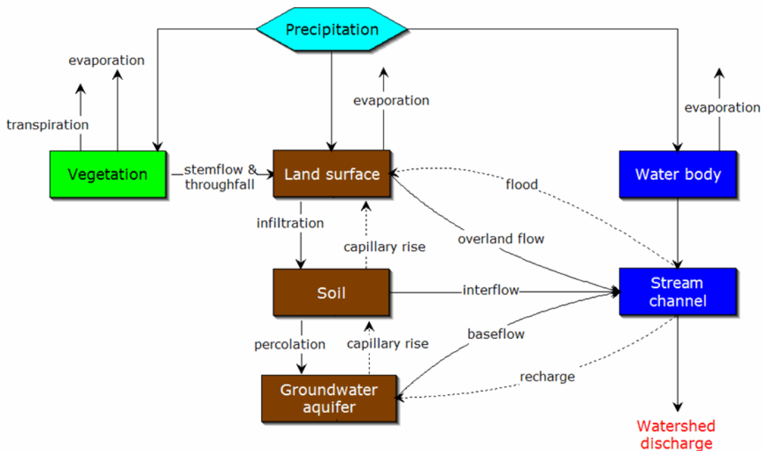
Figure 4-9. Components of the hydrograph method
