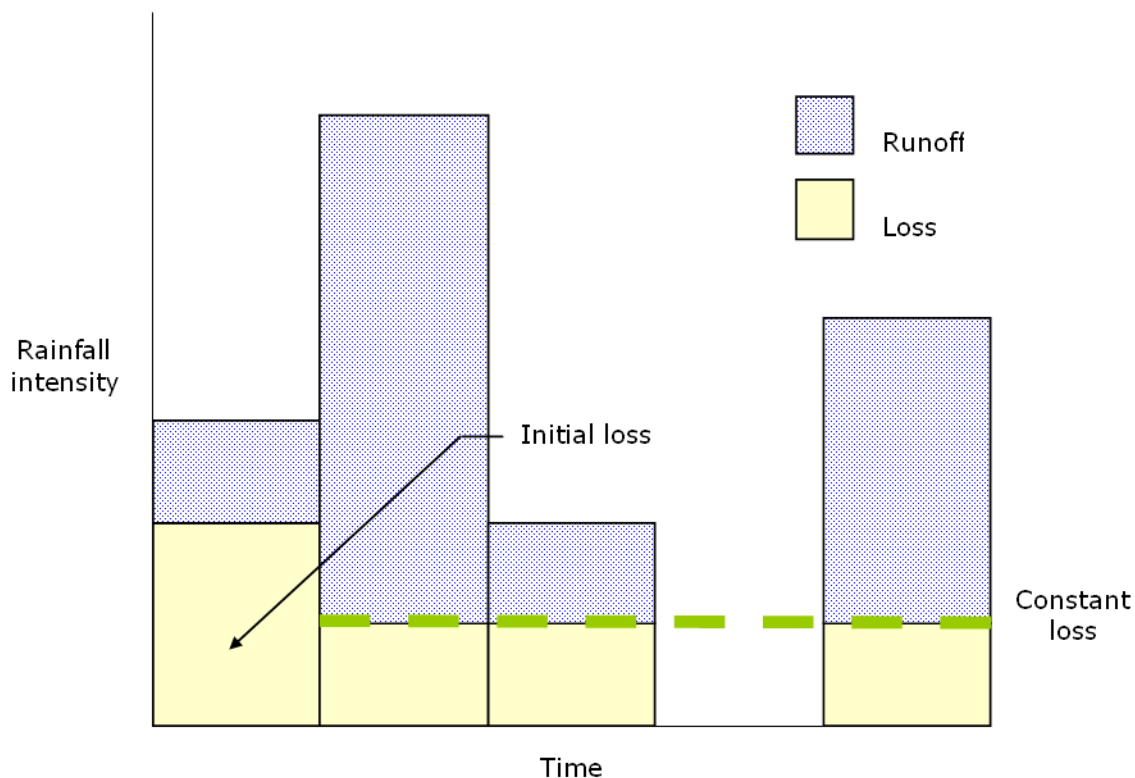
Figure 4-20. Initial and constant-loss rate model
