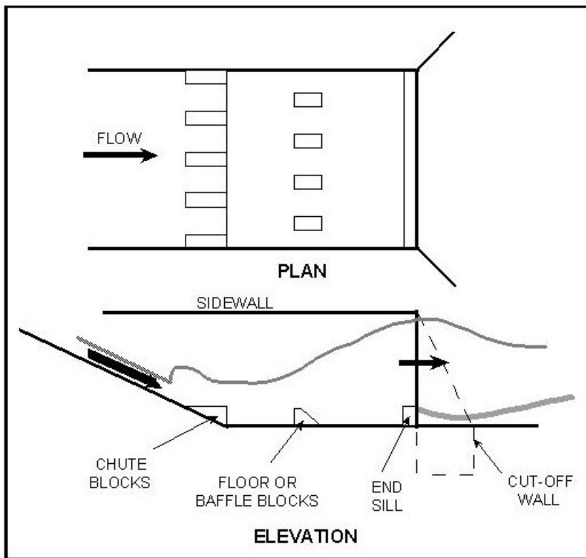
Figure 8-29. Stilling Basins
