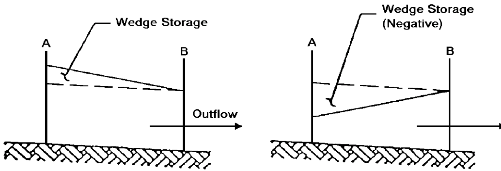
Figure 4-32. Muskingum prism and wedge storage
