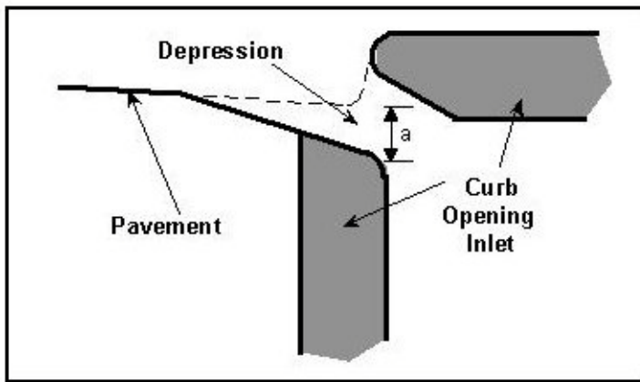
Figure 10-4. Curb Opening Inlet Depression
