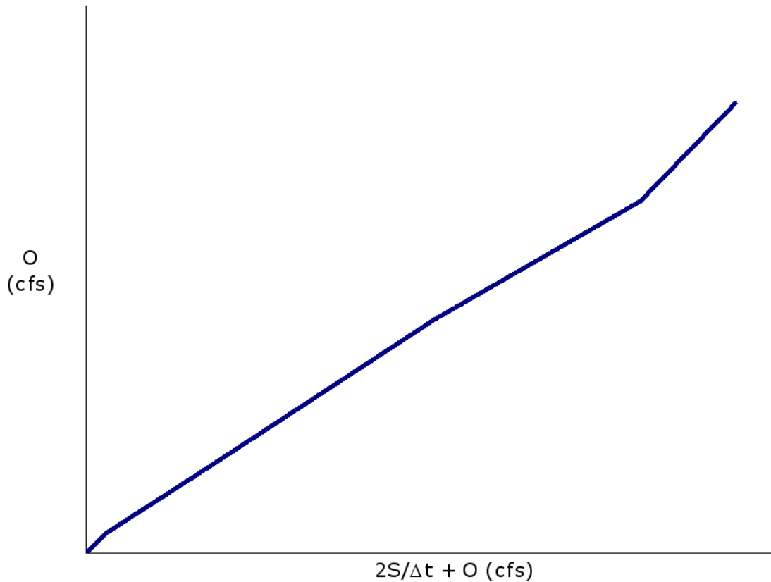
Figure 4-31. Sample storage-indication relation
