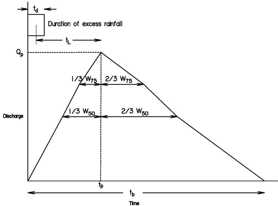
Figure 4-25. Snyder's unit hydrograph
