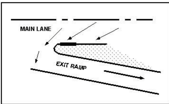
Figure 10-10. Inlet at a Gore Island
