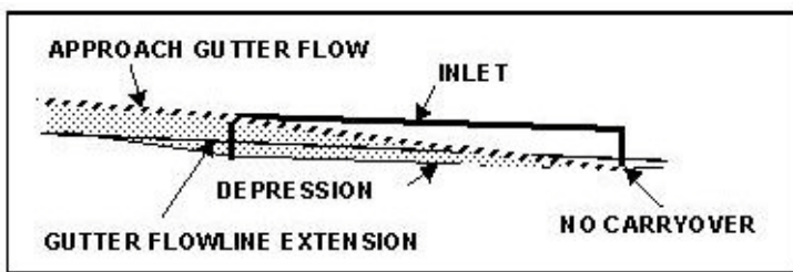
Figure 10-12. Inlet Designed with No Carryover
