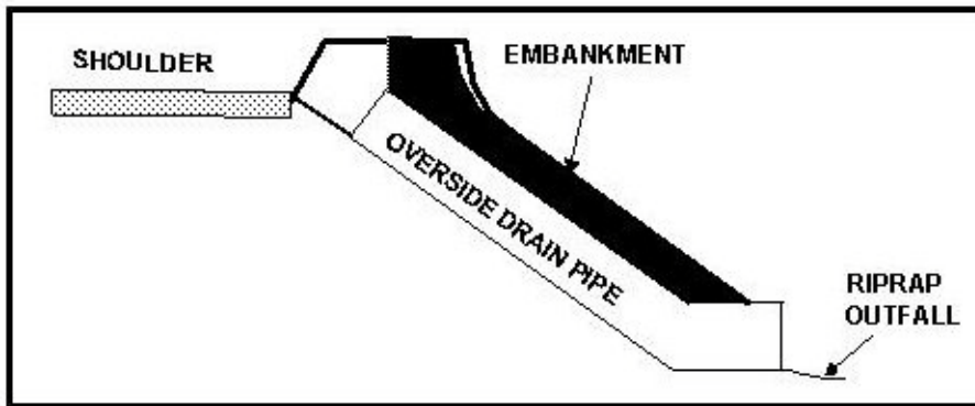
Figure 10-9. Over-Side Drains
