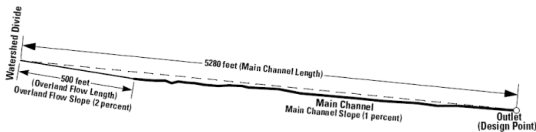
Figure 4-7. Example application of Kerby-Kirpich method
