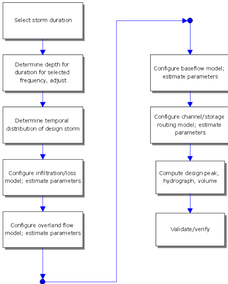
Figure 4-10. Steps in developing and applying the hydrograph method
