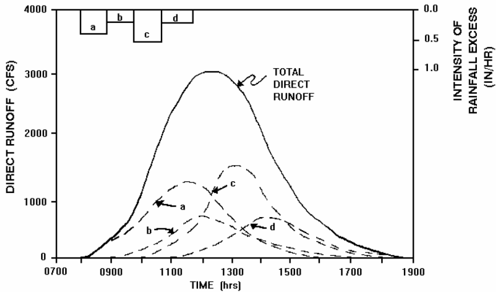
Figure 4-24. Unit hydrograph superposition (USACE 1994)
