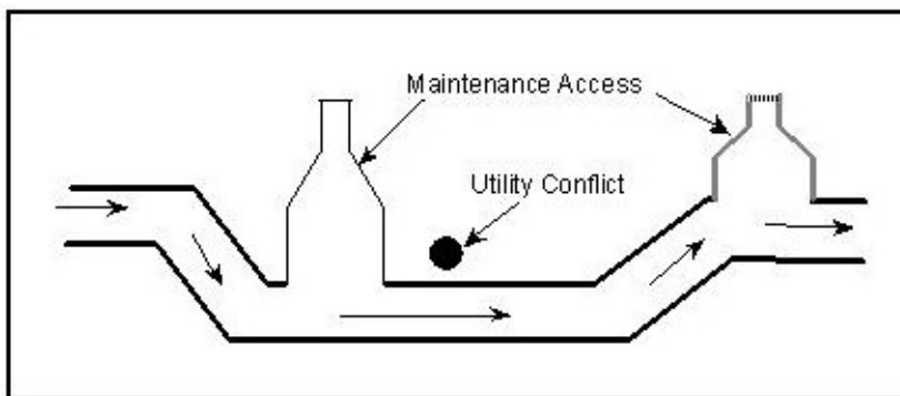
Figure 10-19. Inverted Siphon
