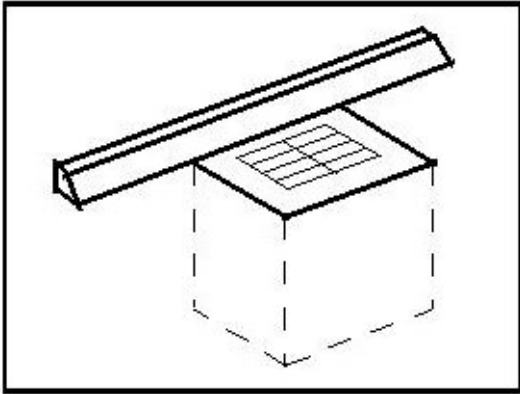
Figure 10-5. Grate Inlet Schematic
