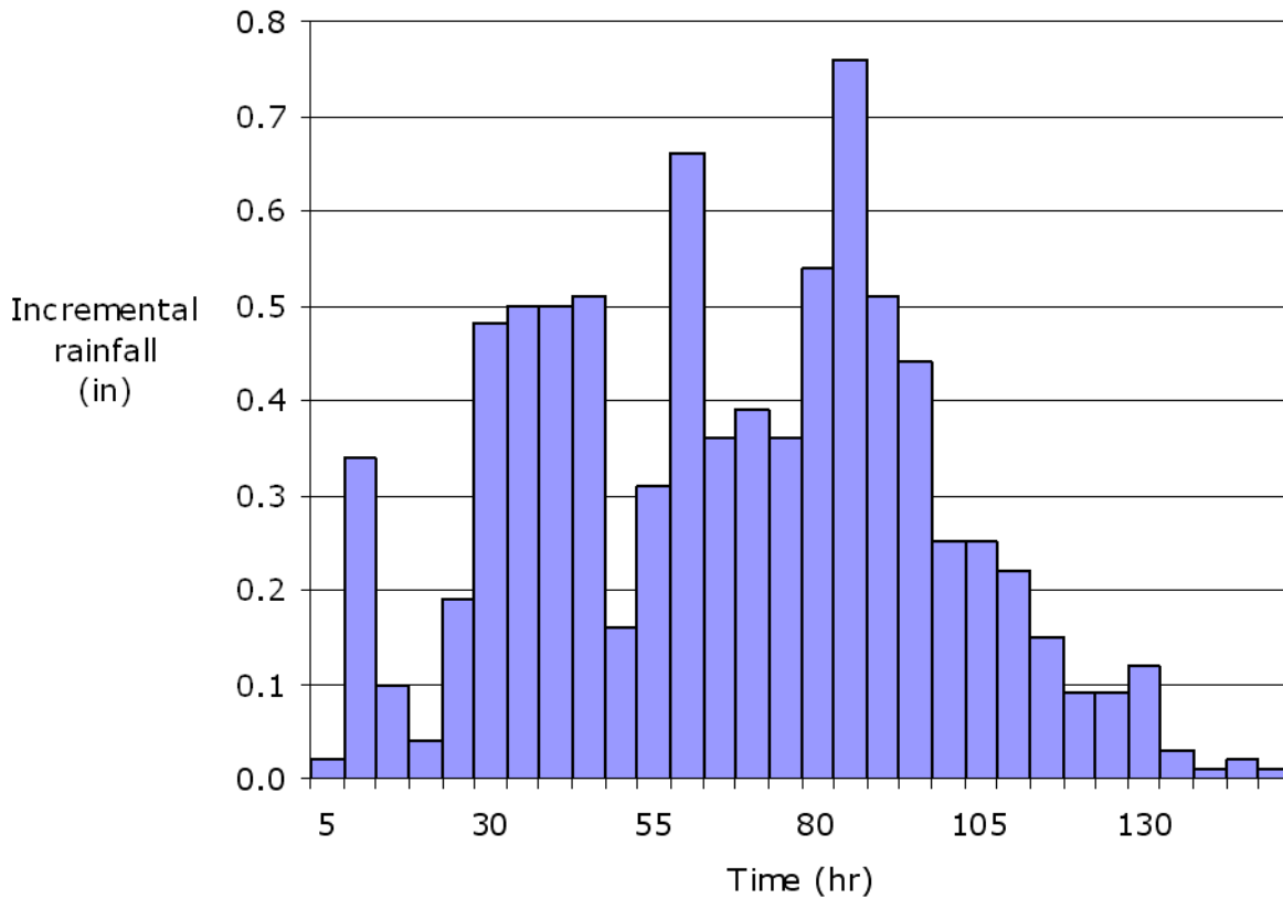
Figure 4-13. Rainfall hyetograph
