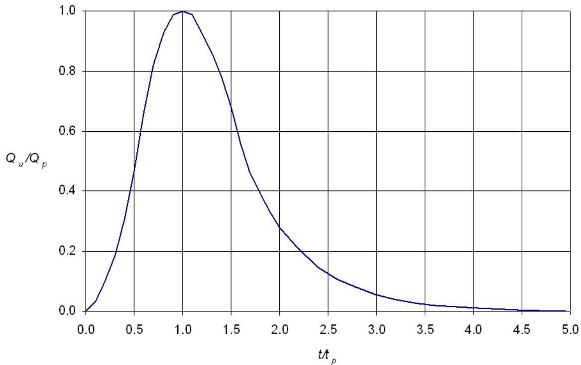
Figure 4-27. Example site-specific unit hydrograph
