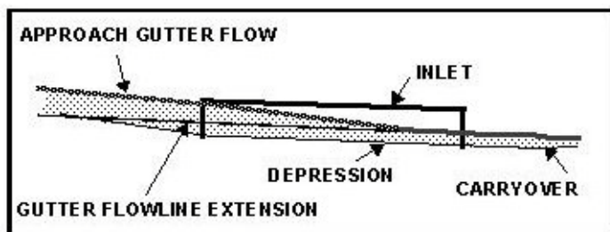
Figure 10-13. Inlet Designed with Carryover
