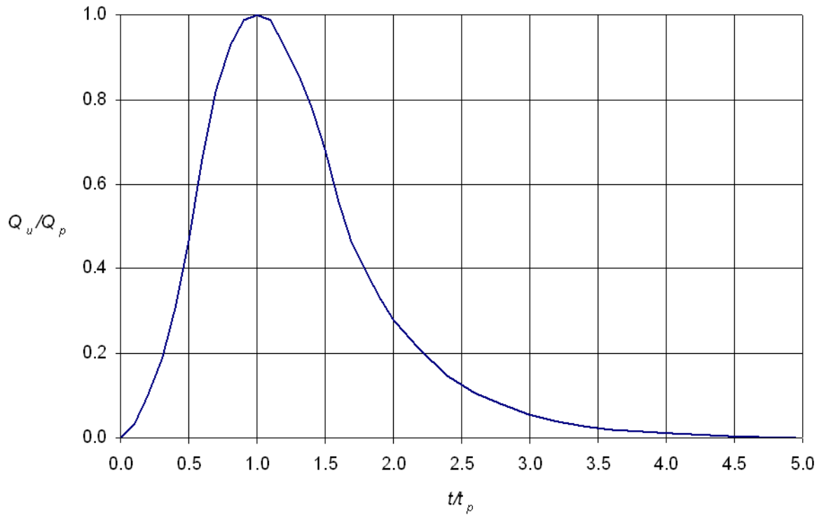
Figure 4-26. NRCS dimensionless unit hydrograph
