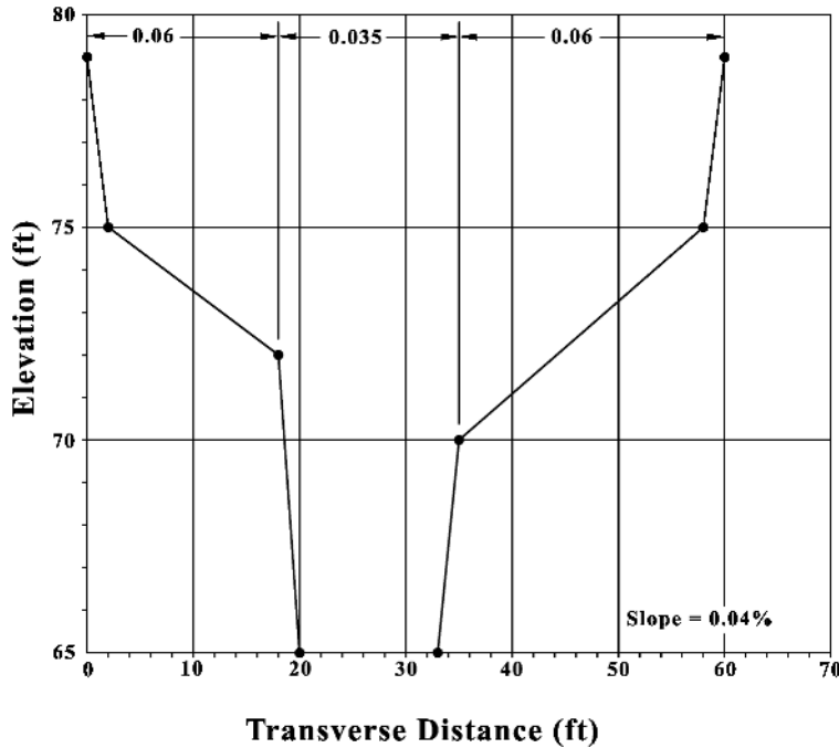
Figure 7-14. Slope Conveyance Cross Section
