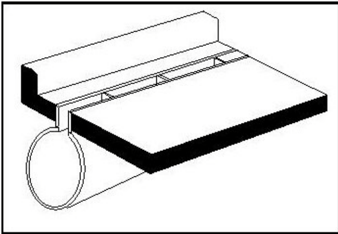
Figure 10-6. Slotted Drain Inlet
