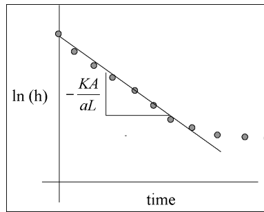
Figure 3: Falling head permeameter results (typical)
