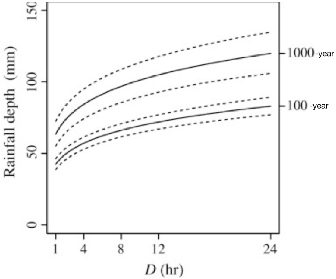
Figure 1: Depth-duration-frequency curve
