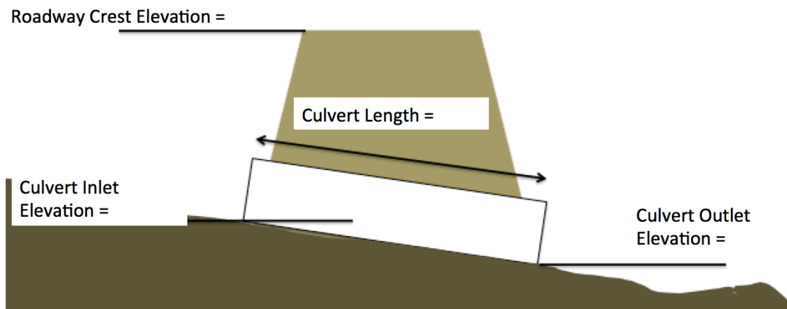
Figure 5: Culvert system elevation view sketch
