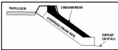
Figure 10-8. Over-Side Drains
