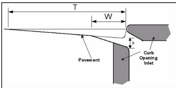
Figure 10-14. Gutter Cross-Section Diagram
