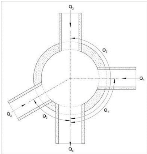
Figure 10-22. Access hole angled inflow definition.
