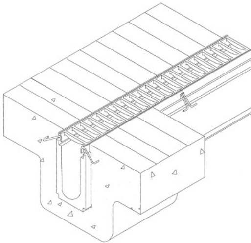
Figure 10-6. Precast trench drain.
