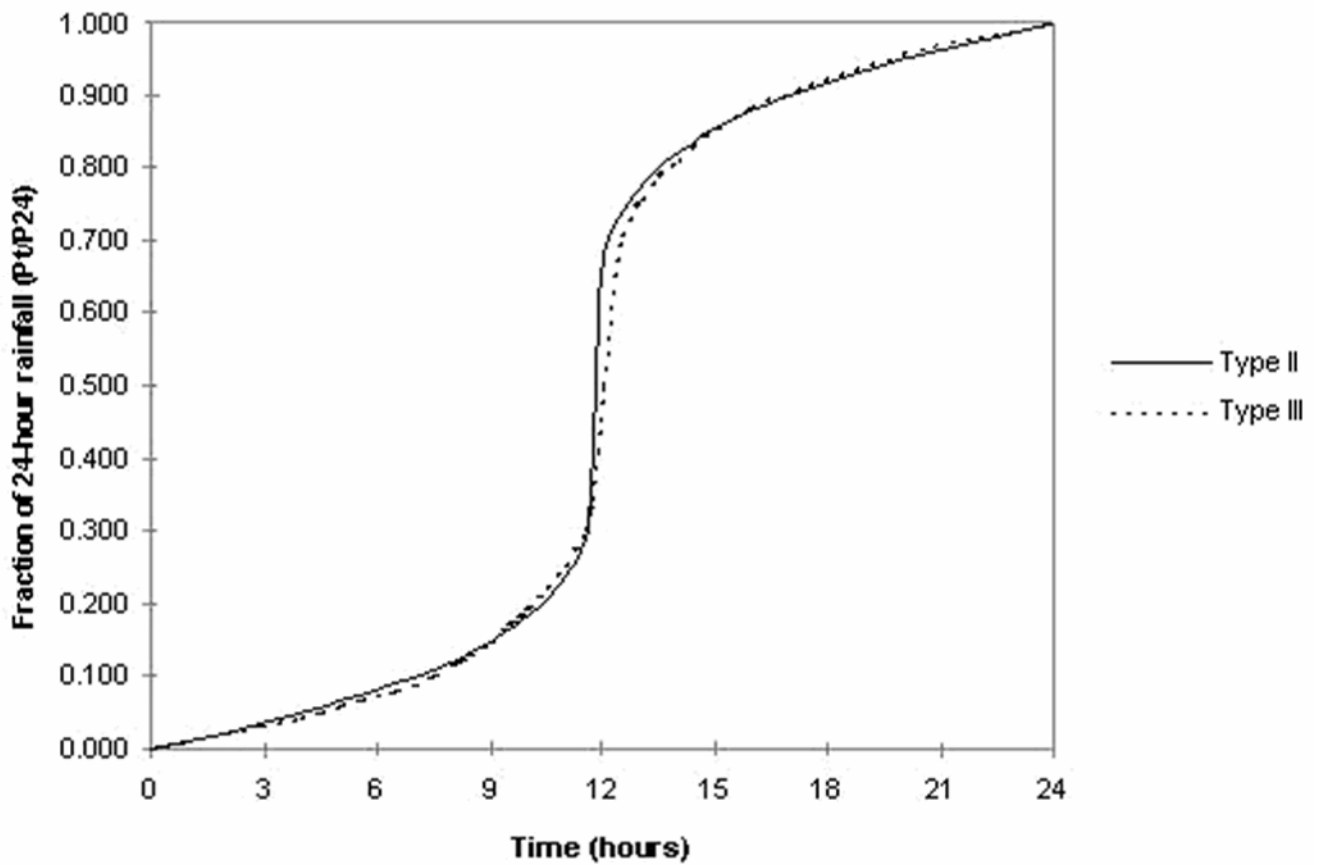
Figure 4-14. NRCS 24-hour rainfall distributions (NRCS 1986)
