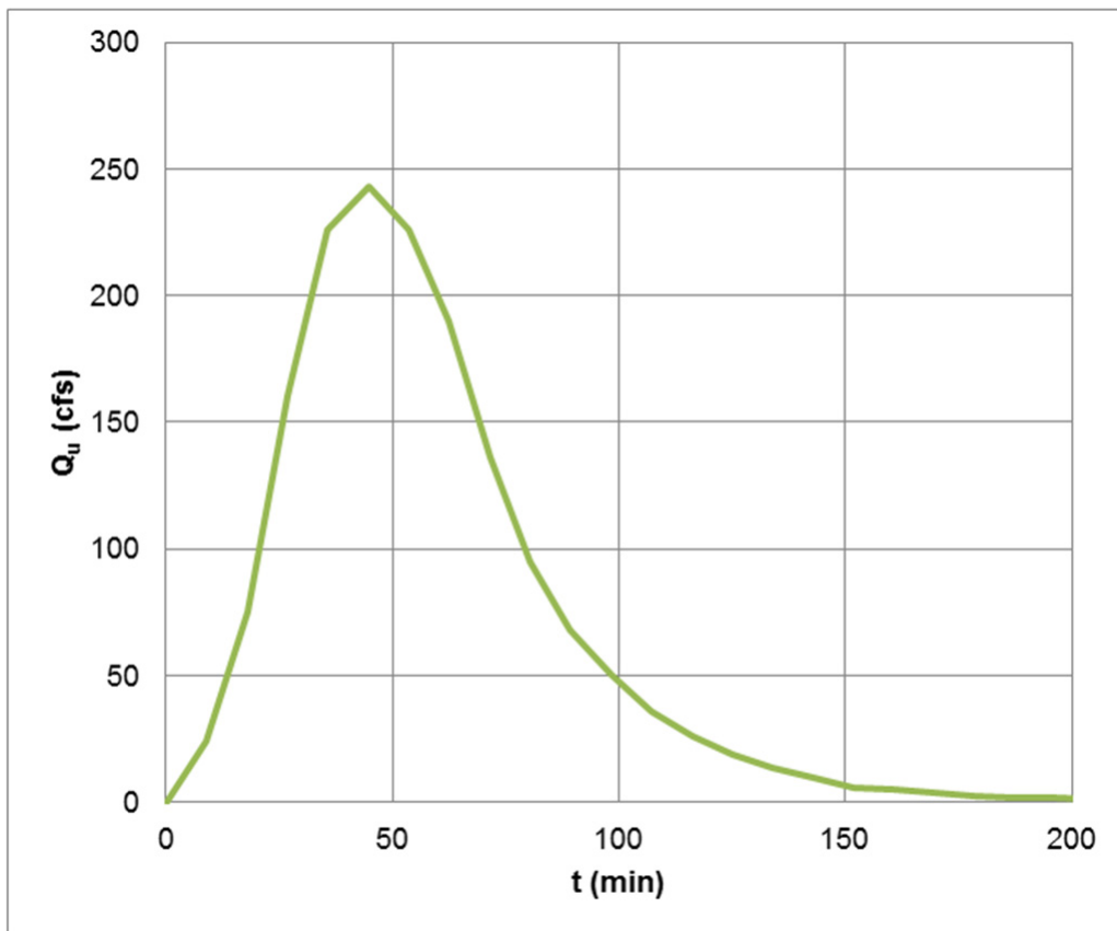
Figure 4-27. Example site-specific unit hydrograph
