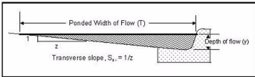
Figure 10-10. Gutter Flow Cross Section Definition of Terms
