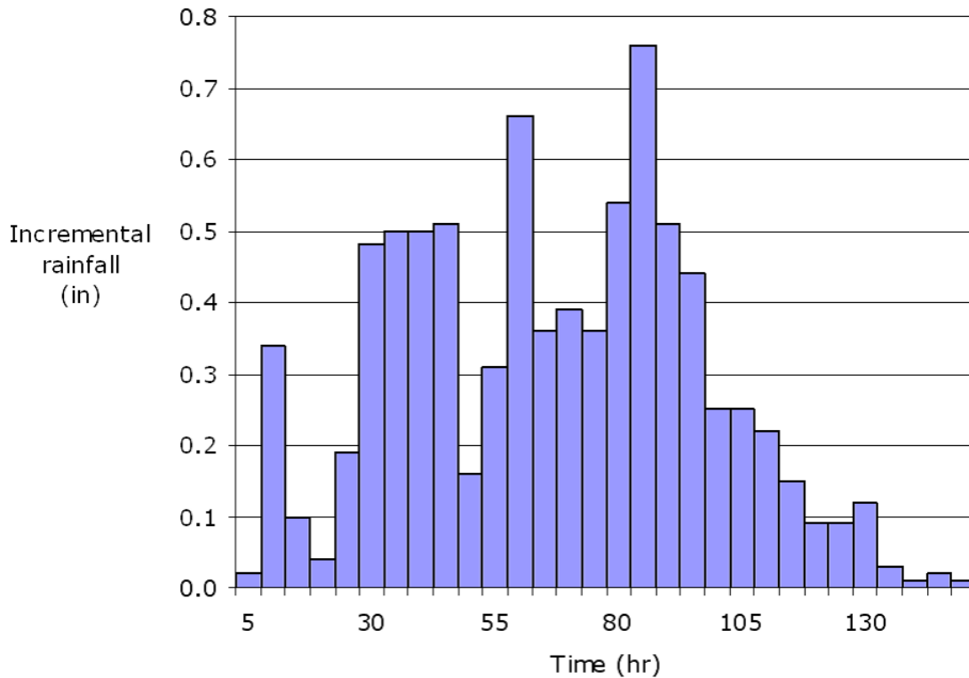
Figure 4-13. Rainfall hyetograph
