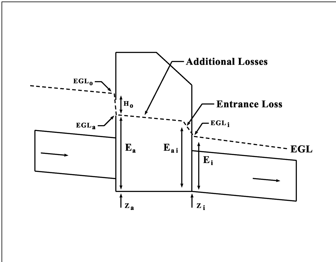
Figure 10-20. Access Hole Energy Level Definitions
