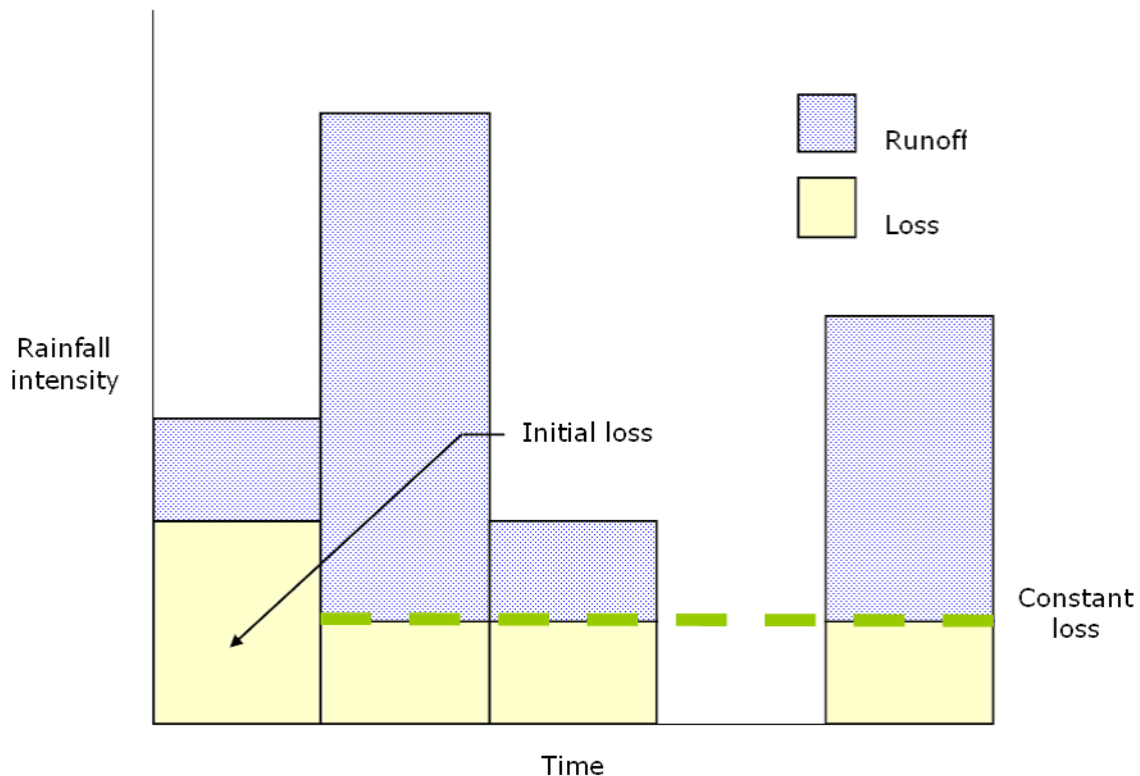
Figure 4-20. Initial and constant-loss rate model
