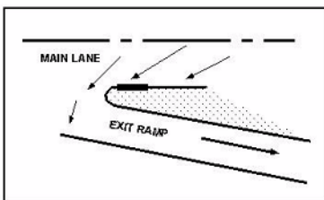
Figure 10-9. Inlet at a Gore Island
