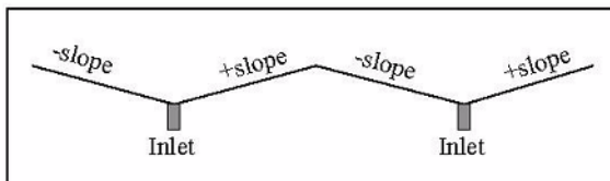
Figure 10-1. Rolling Gutter Profile
