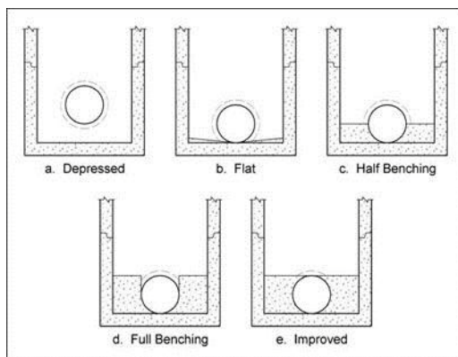
Figure 10-21. Access hole benching methods
