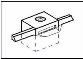
Figure 10-2. Curb Opening Inlet
