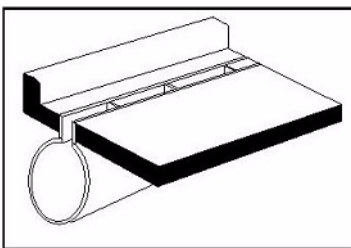
Figure 10-5. Slotted Drain Inlet
