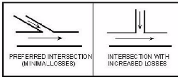
Figure 10-18. Acute Angle and Right Angle Intersections
