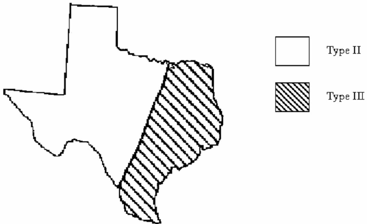
Figure 4-15. Rainfall distribution types in Texas (TR-55 1986)
