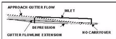
Figure 10-12. Inlet Designed with No Carryover
