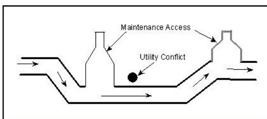
Figure 10-19. Inverted Siphon
