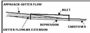
Figure 10-13. Inlet Designed with Carryover
