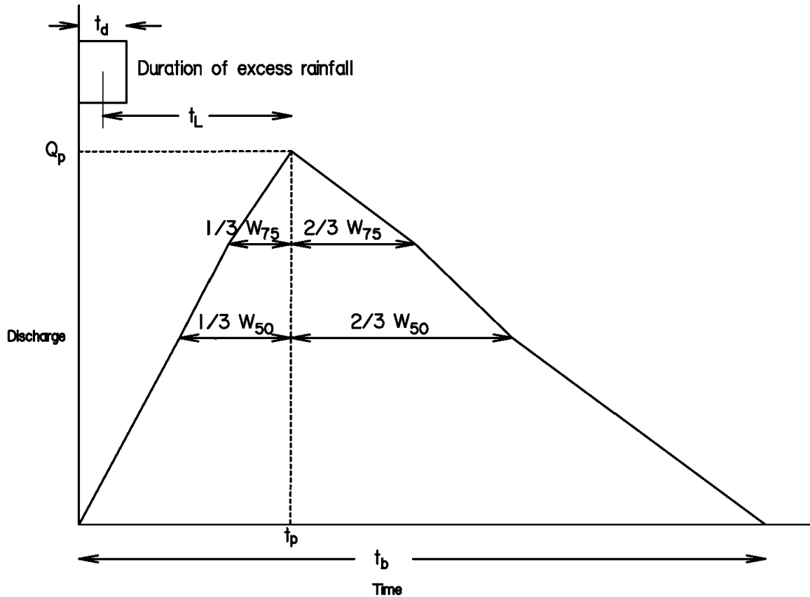
Figure 4-25. Snyder's unit hydrograph
