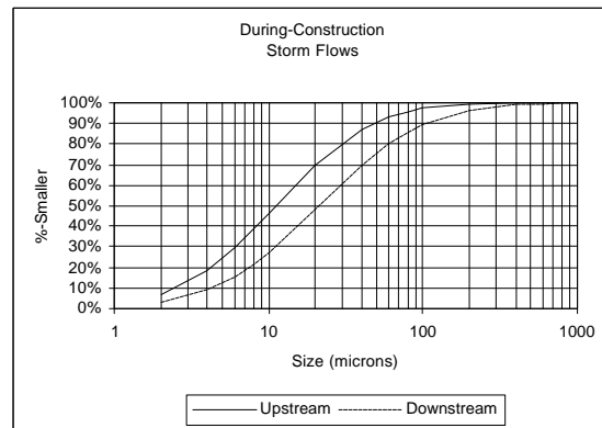
Figure 11: PSD during construction, upstream versus downstream (storm)
