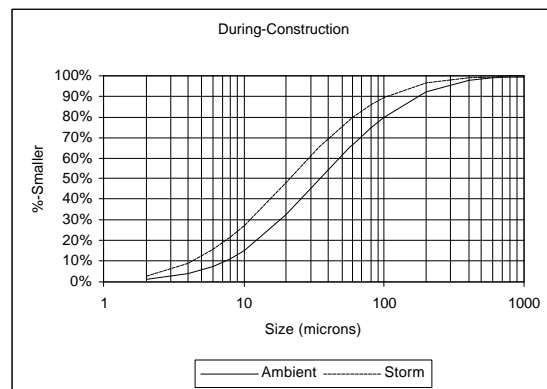
Figure 9: PSD during construction downstream of TSC
