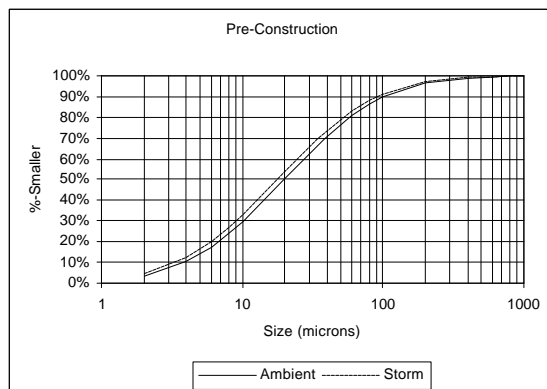
Figure 8: PSD preconstruction downstream of TSC
