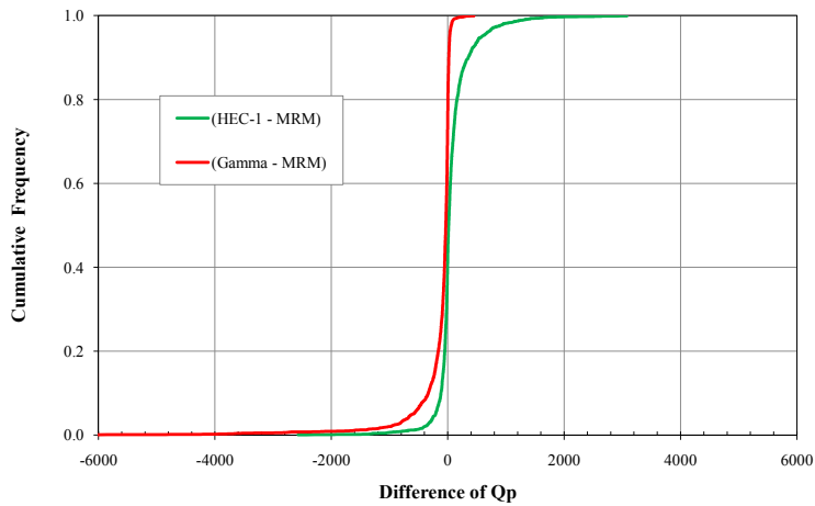
Figure D.13: Cumulative distributions of differences of simulated Q_p between different methods. The green curve is for differences of simulated Q_p between Clark and MRM unit hydrographs, and the red curve is for differences of simulated Q_p between gamma and MRM unit hydrographs.
