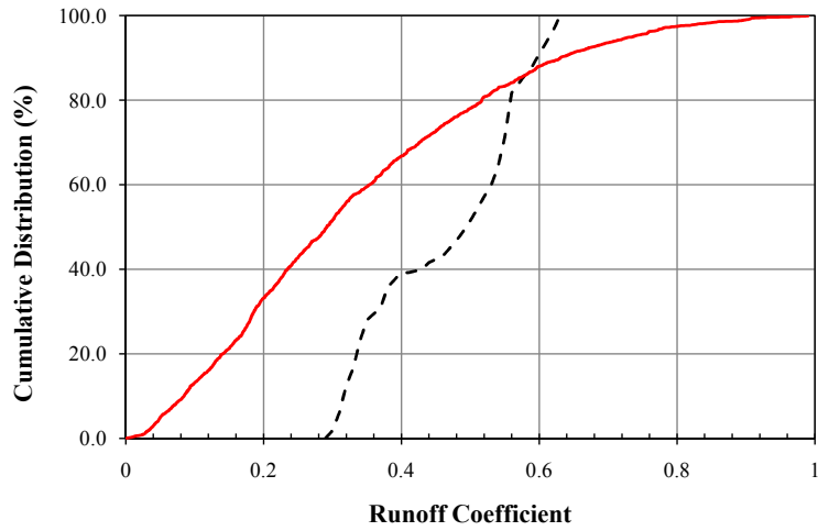
Figure 2.6: Cumulative distributions of the runoff coefficients C_v^{bc} (solid) and C_v^{lit} (dashed).
