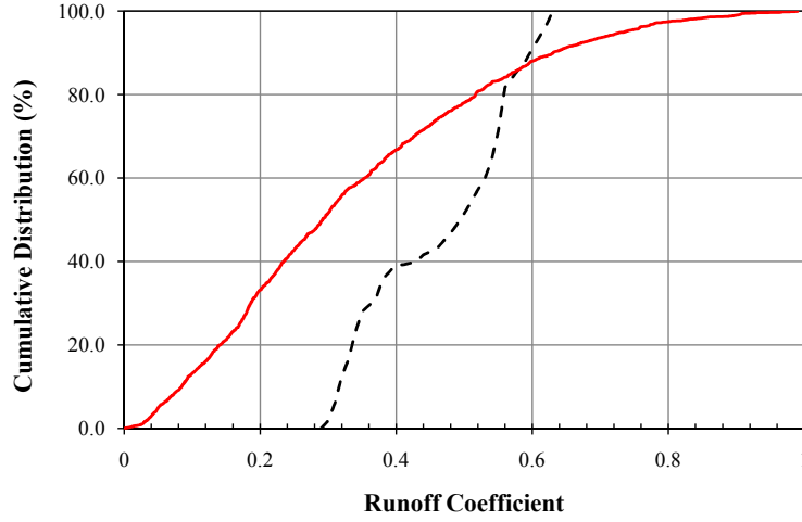
Figure D.1: Cumulative distributions of the runoff coefficients C_v^{\text{bc}} (red) and C_v^{\text{lit}} (black).
