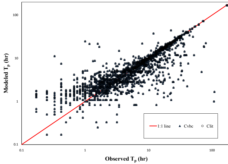
Figure D.6: Modeled and observed time to peak from C_v^{bc} (blue) and C_v^{lit} (black) with timing parameters from the Kerby-Kirpich method.
