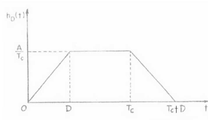
Figure 2.5: The D -hour unit hydrograph of the rational method for D < T_c (Singh and Cruise, 1992).
