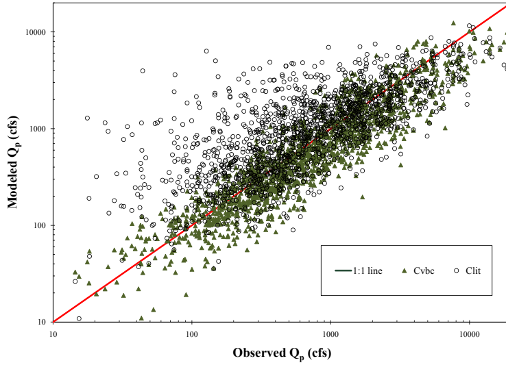
Figure D.5: Modeled and observed peak discharge from C_v^{bc} (green) and C_v^{lit} (black) with timing parameters derived from the Kerby-Kirpich method.
