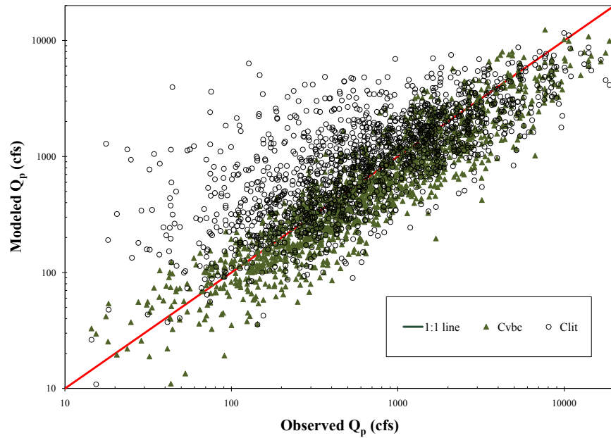
Figure 2.7: Modeled and observed peak discharge from C_v^{bc} (solid triangle) and C_v^{lit} (open circle) with timing parameters derived from the Kerby-Kirpich method.
