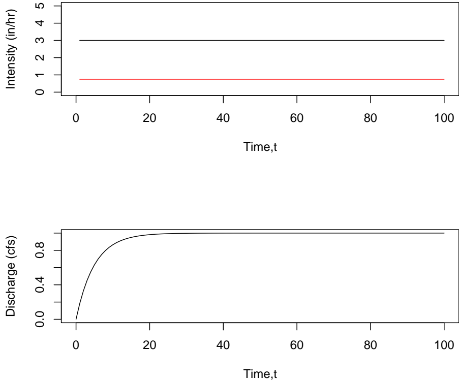
Figure A.1: Runoff generation in rational model. The red line in the upper panel is the excess rainfall intensity, the product of C_{std} , and the raw rainfall intensity. The runoff in the lower panel reaches equilibrium at about 20 time units. The rational method only identifies the equilibrium discharge and does not necessarily produce the shape leading to equilibrium in this diagram.
