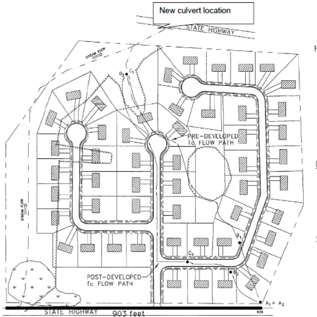
Figure 4.1: Subdivision X Drainage to a Highway Culvert
