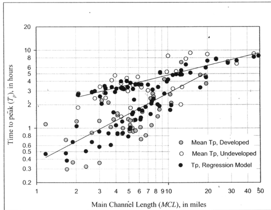
Fig. 4. Plot of relation between observed T_p of 1-minute unit hydrograph and main channel length for undeveloped and developed watersheds.
