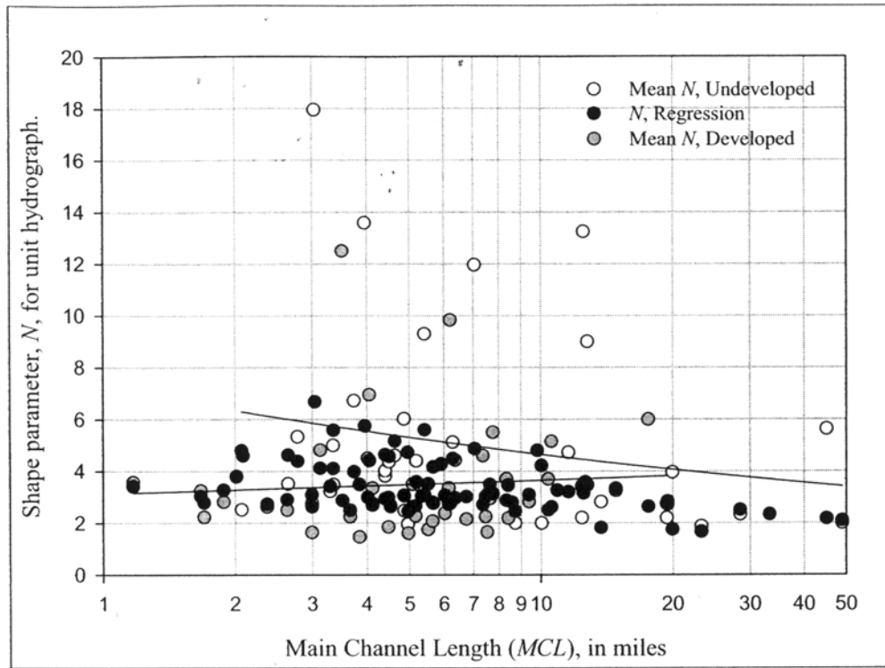
Fig. 3. Plot of relation between observed N of 1-minute unit hydrograph and main channel length for undeveloped and developed watersheds.
