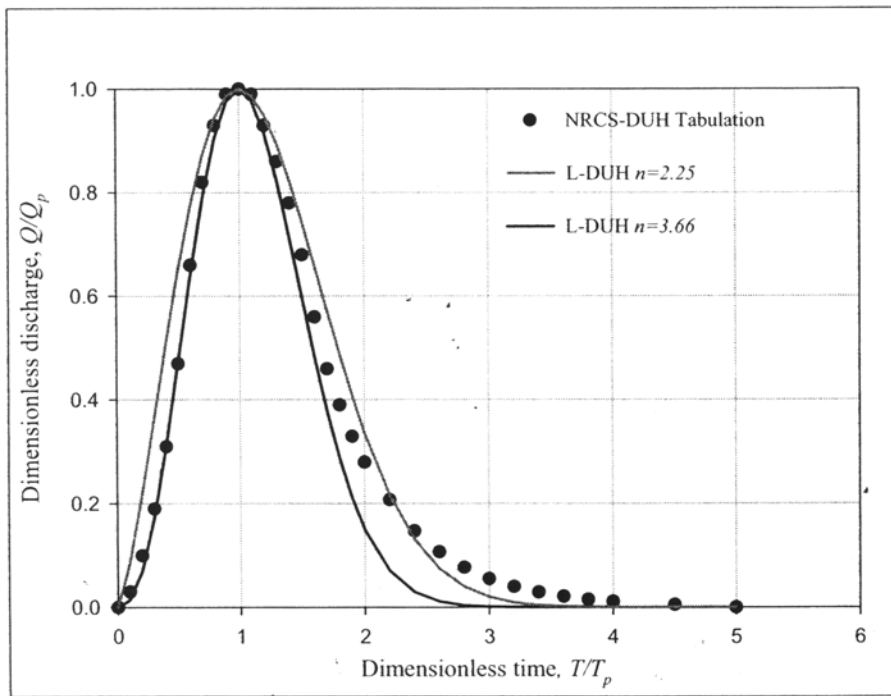
Fig. 2. NRCS DUH and Leinhard DUH (L-DUH). N=3.66 is mean value applicable for the study watersheds.
