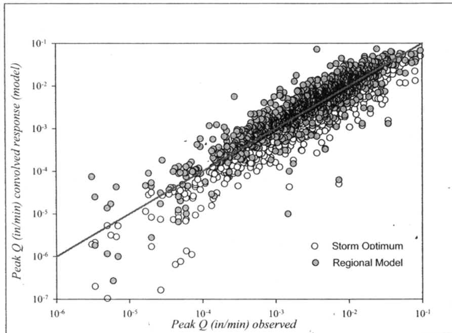
Fig. 5. Plot of relation between peak discharge from convolution of observed rainfall versus observed peak discharge.
