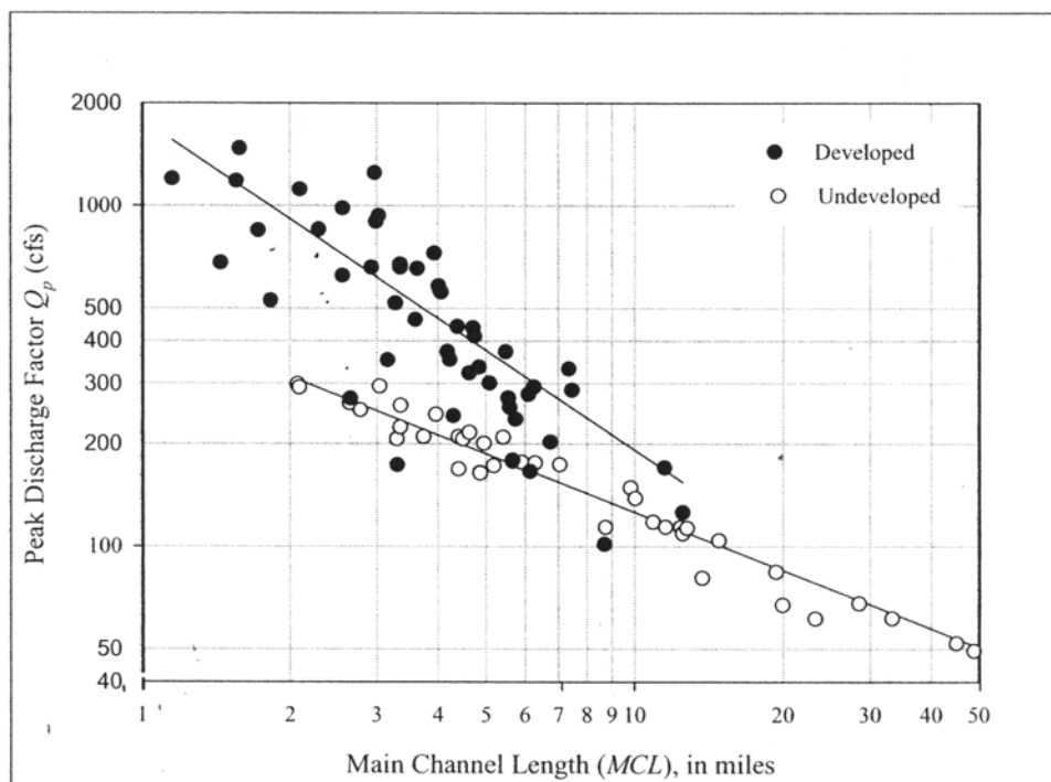
Fig. 6. Plot of relation of Q_p and main channel length for undeveloped and developed watersheds.
